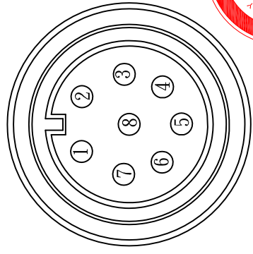
P3 Pin Assignments Front View
