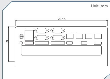
FB11 DS-1001 Front Bezel with 4x RJ45 Dimension (WxD) : 207.5 x 89 mm
