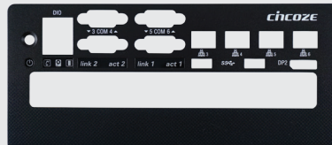
FB11 DS-1001 Front Bezel with 4x RJ45 Dimension (WxD) : 207.5 x 89 mm
