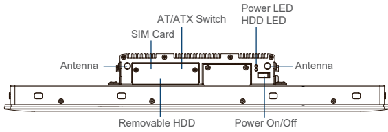
Front I/O
