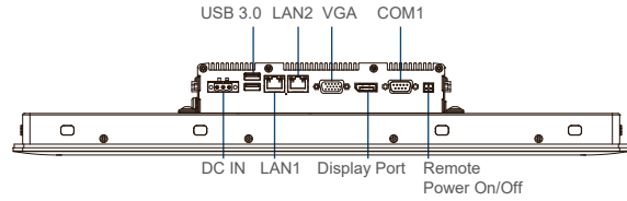
Rear I/O
